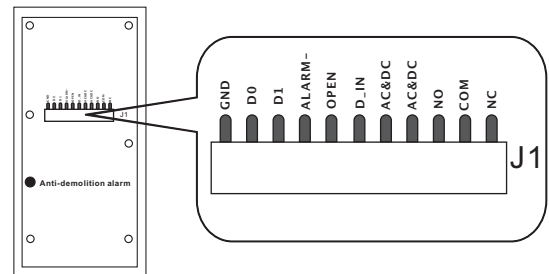
PCB connect diagram
